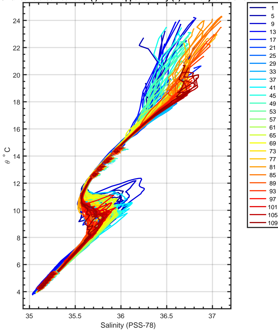
6901262 uncalibrated float data (-) and mapped salinity (o) with objective errors
