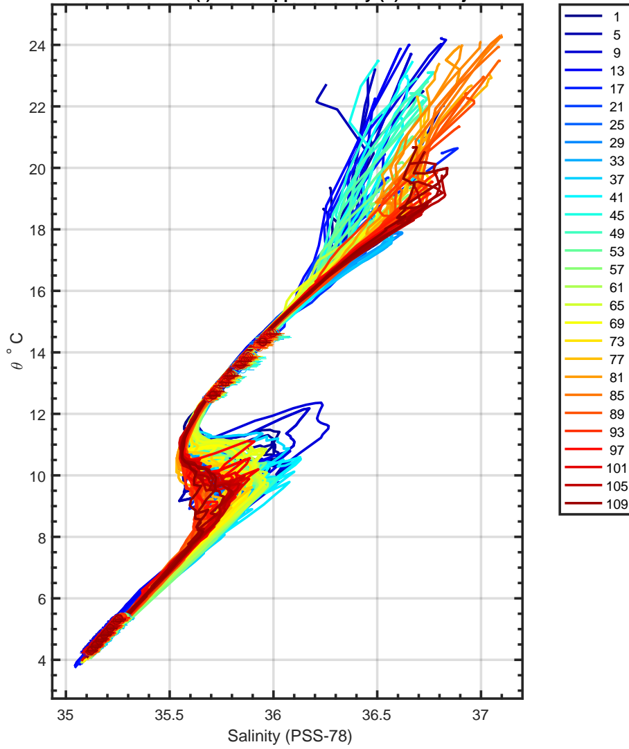
6901262 calibrated float data (-) and mapped salinity (o) with objective errors
