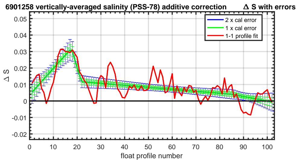
Figure 7: Salinity variation between each profile. Owens and Wong Objective Mapping Analysis builds its model based in a programmed number of break points.
