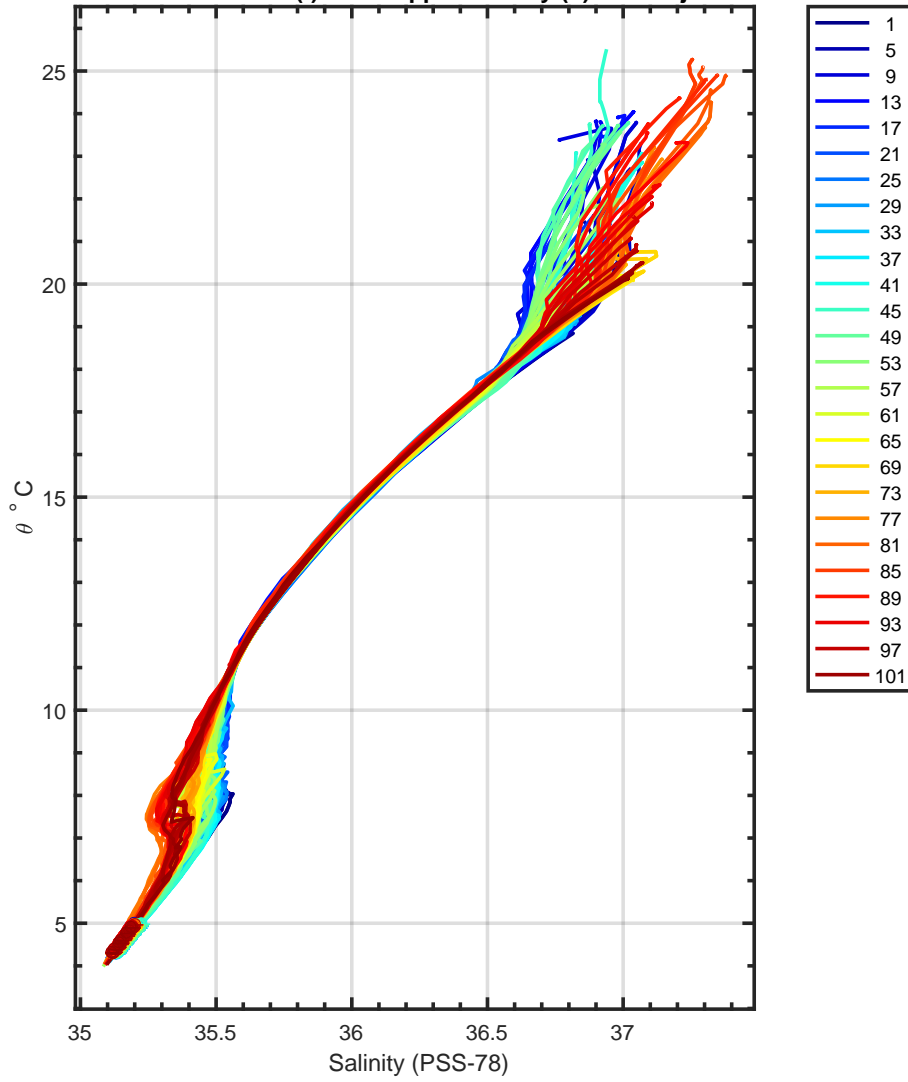
6901258 uncalibrated float data (-) and mapped salinity (o) with objective errors
