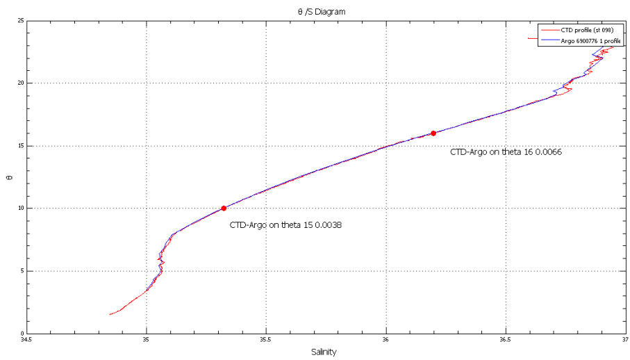
Figure 10: Salinity difference between CTD profile and ARGO profile. The theta variation points are pointed out.
