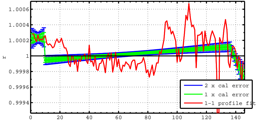
6900775 potential conductivity (mmho/cm) multiplicative correction r with error
