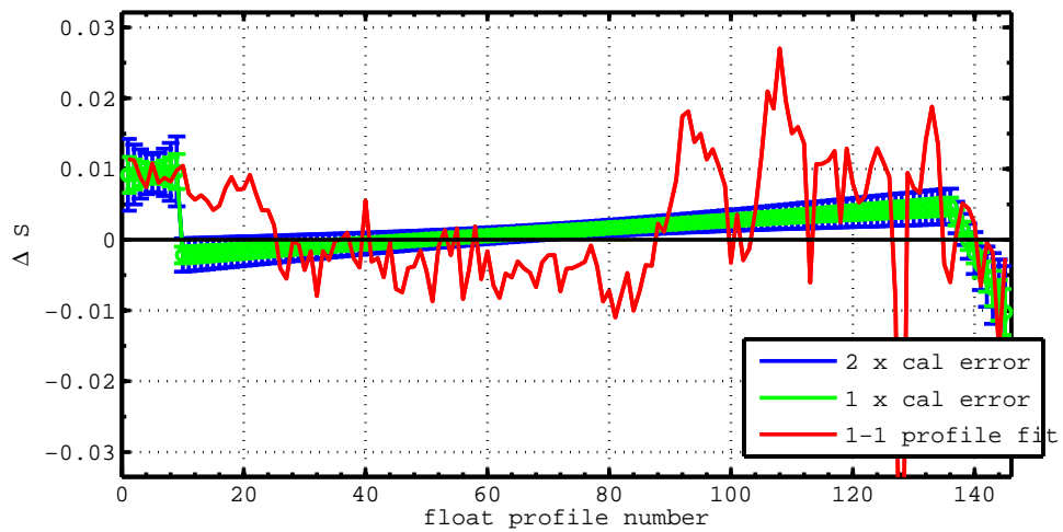
6900775 vertically-averaged salinity (PSS-78) additive correction \Delta S with error
