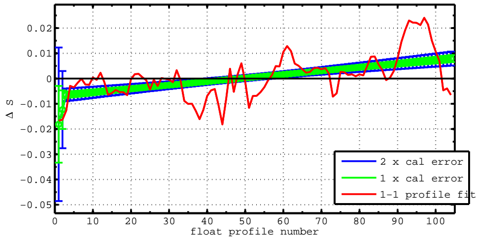
6901241 vertically-averaged salinity (PSS-78) additive correction \Delta S with error
