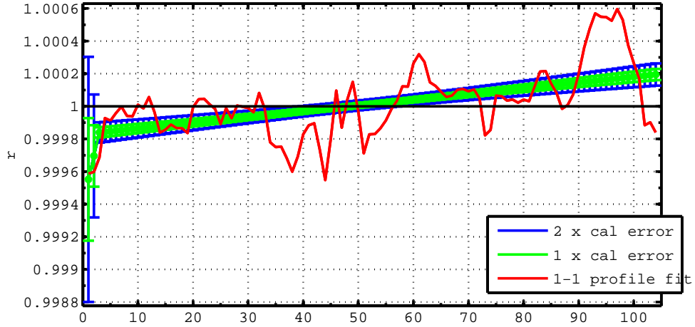
6901241 potential conductivity (mmho/cm) multiplicative correction r with error
